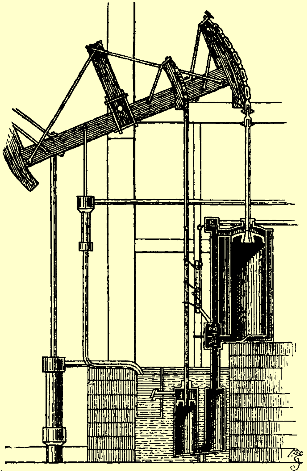
THE ENGINE BEELZEBUB, 1767.
